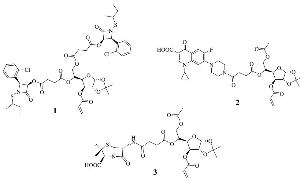
Figure 1. Glycosylated antibiotic acrylates used for the formation of glyconanobiotics: bis- N - sec -butylthio \beta -lactam acrylate (1), ciprofloxacin acrylate (2), 6-aminopenicillanic acid acrylate (3).
