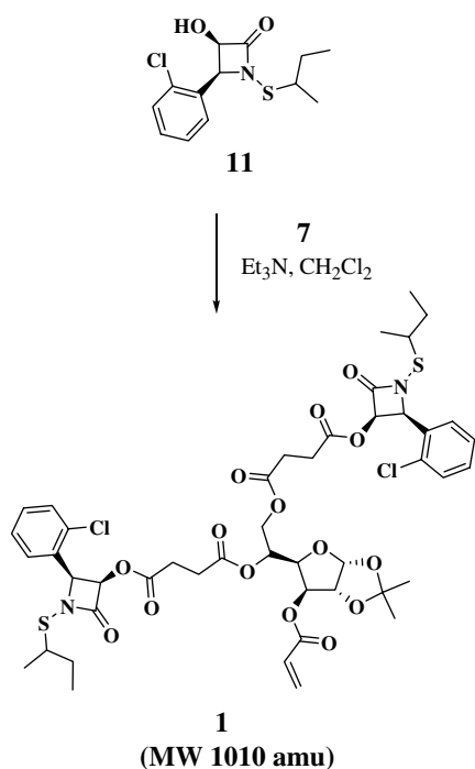
Scheme 3. Synthesis of bis- N - sec -butylthio β-lactam acrylate ( 1 ).
